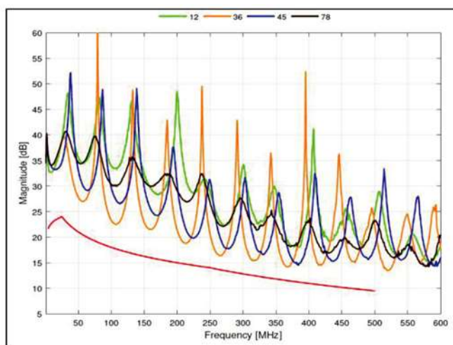
Typical Return Loss CAT.6A UTP patch cord
