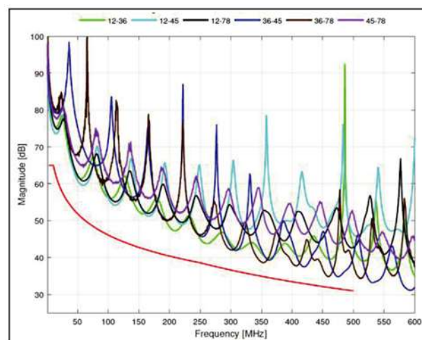
Typical NEXT CAT.6A UTP patch cord
