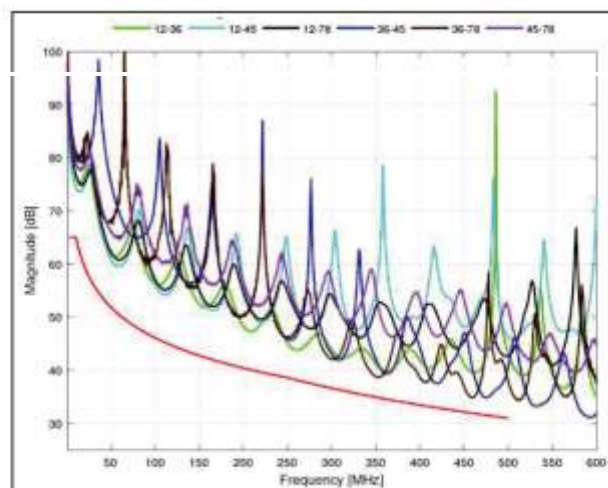
Typical NEXT CAT.6A S/FTP patch cord
